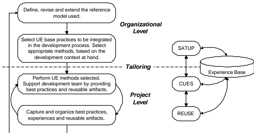
Figure 1 : Tool Support for Evidence-Based Usability Engineering
